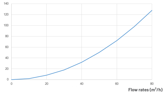
Pressure losses (mBar)
